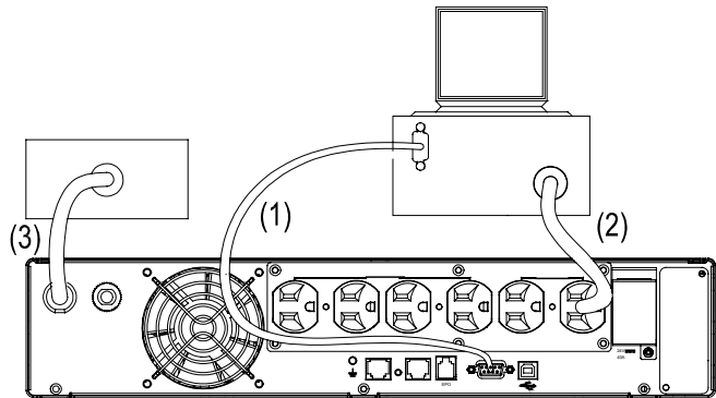
Figure 3-4 UPS Connector for 1KVA
