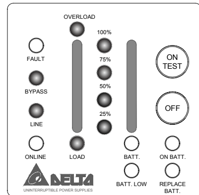
Figure 3-9 Overload and UPS turn into Bypass
