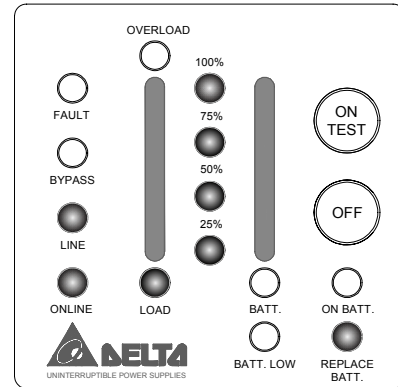
Figure 3-10 Battery Replace
