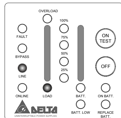
Fig 3-5 Stand-By Mode
