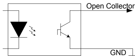
Figure 4-2 Open Collector Circuit
