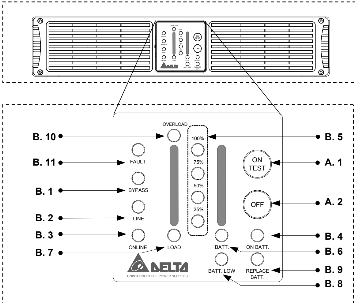
Figure 2-1 Operation Panel
